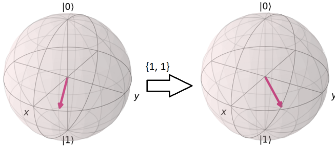
FIGURE 3 A snapshot of rotating the qubit using the brain code \{1, 1\} .
